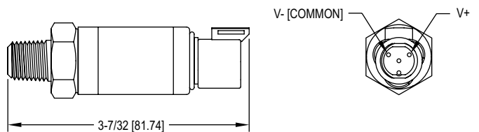
Figure P: Deutsche connection
