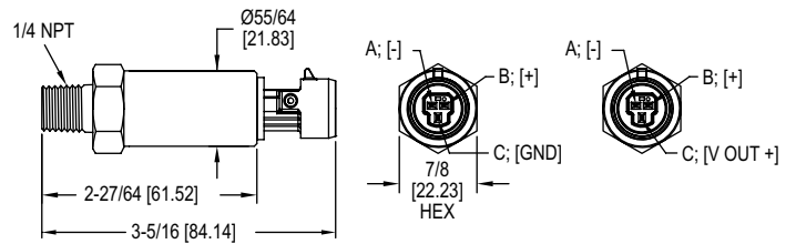
Figure F: Packard connection
